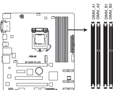
B150M-PLUS 288-pin DDR4 DIMM sockets
