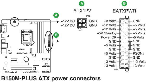
B150M-PLUS ATX power connectors
